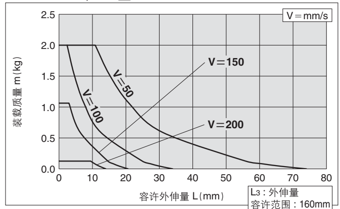
MXQ8B-40、50Z□
